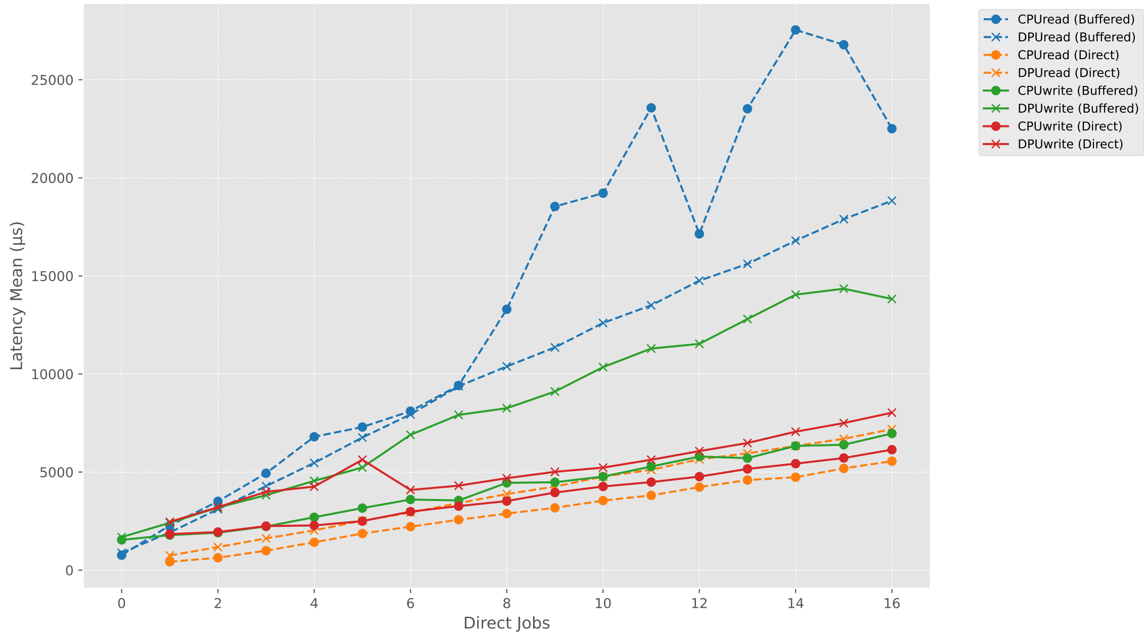
Latency Mean vs Direct Jobs (buffered1_directN) - SEQ (CPU vs DPU)
